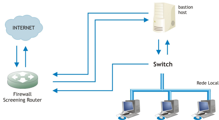
Figura 14 – Screened host
