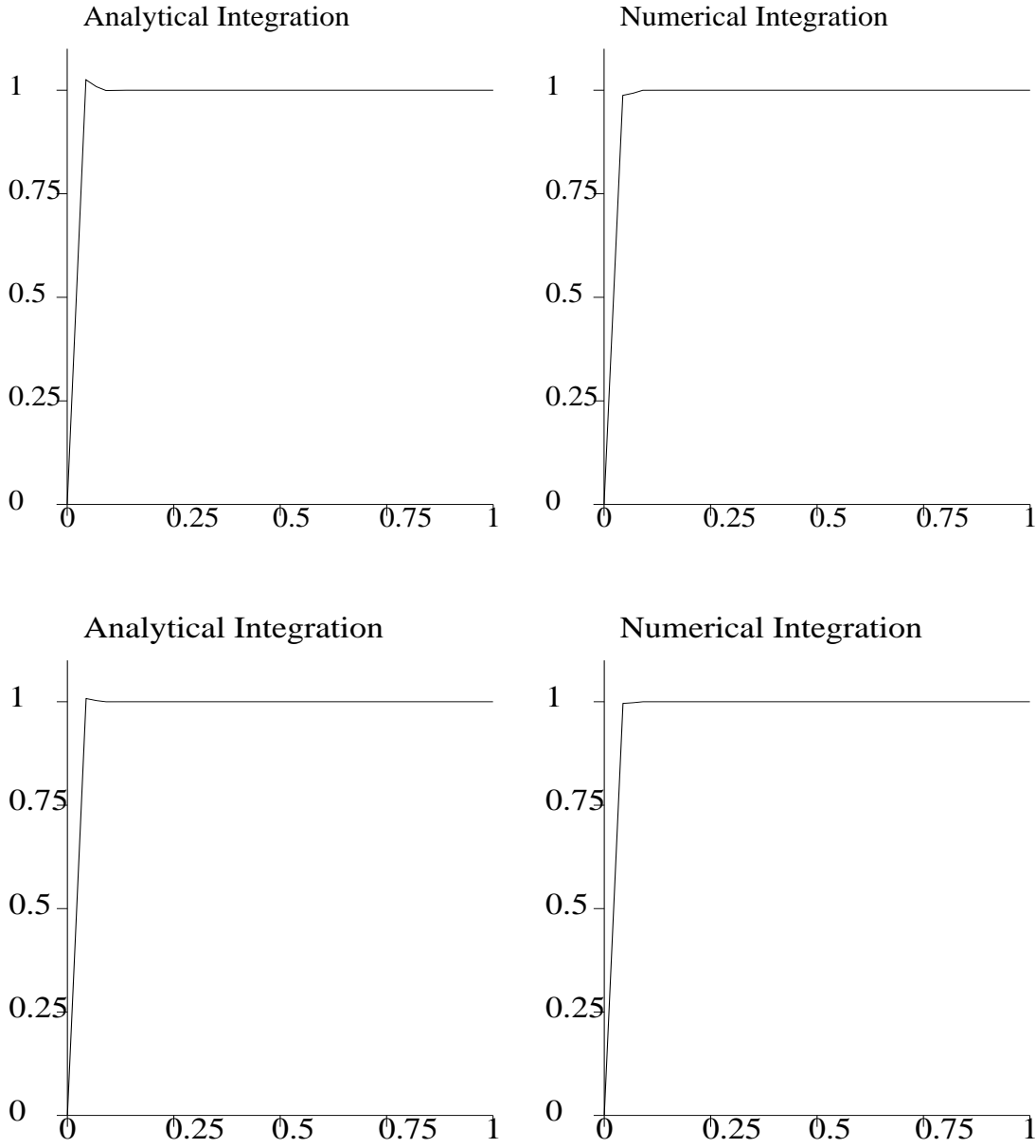
Fig. 4. Profile of solutions at y = 1/2 , using numerical and analytical integration adopting \sigma = 1 and \varepsilon = 10^{-5} (top) and \varepsilon = 10^{-6} (below).
